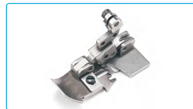
名称: 压脚组件 (厚料) Description: Presser Foot (Heavy Duty) 代 码/Part NO: 2061604000 适 配: E4/C3/C4/C5系列 A04/435机型, E3-5×2-56 Machine Type: A04/435 type for E4/C3/C4/C5 series, E3-5×2-56
