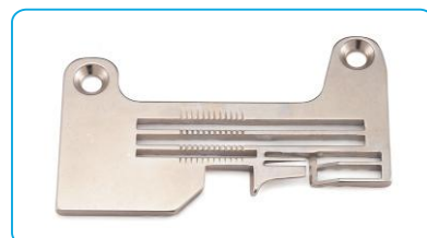
名称: 针板 Description: Needle Plate 代码/Part NO: 20715201 适配: C3/C4/JK-798TE Machine Type: C3/C4/JK-798TE
